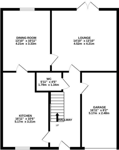
GROUND FLOOR 791 sq.ft. (73.5 sq.m.) approx.
