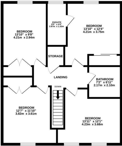
1ST FLOOR 791 sq.ft. (73.5 sq.m.) approx.
