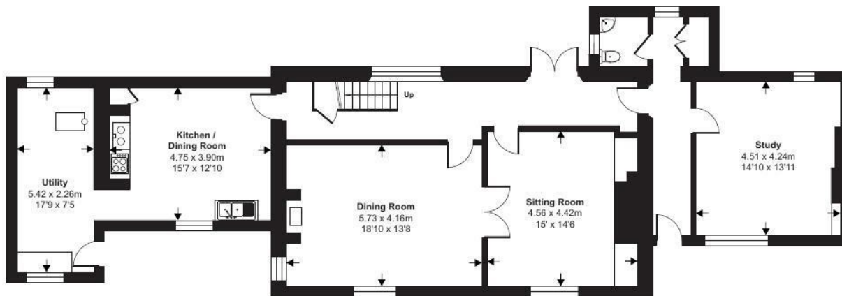
Ground Floor
