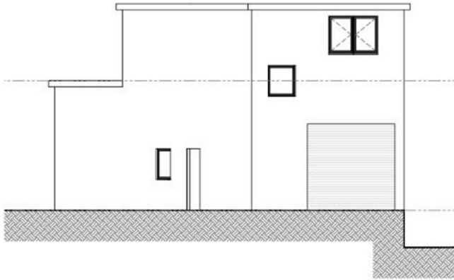
④ North Elevation (Front) - Proposed Scale: 1/50 A2 / 1:500 A3
