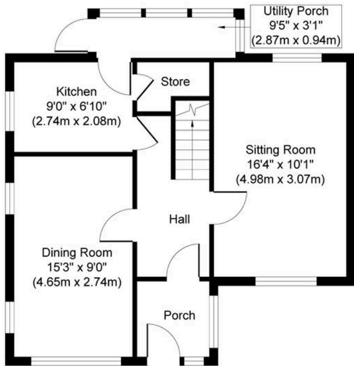
Ground Floor Approximate Floor Area 545 sq. ft (50.60 sq. m)
