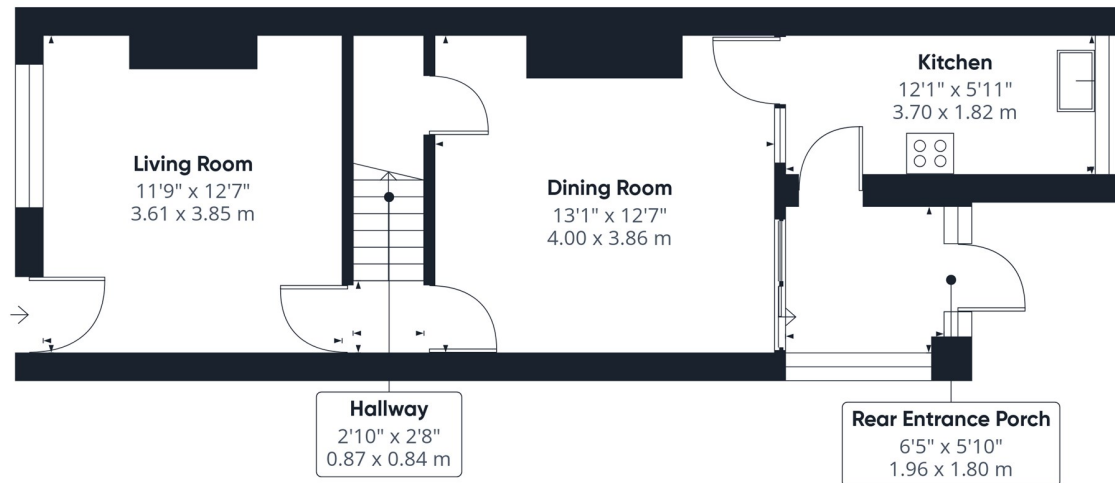
Floor 0
