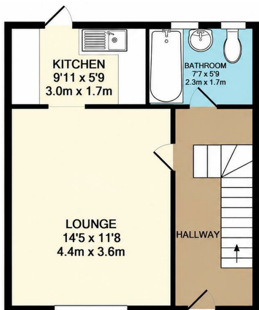
GROUND FLOOR APPROX. FLOOR AREA 352 SQ.FT. (32.7 SQ.M.)
