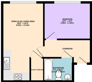
GROUND FLOOR 417 sq.ft. (38.8 sq.m.) approx.
