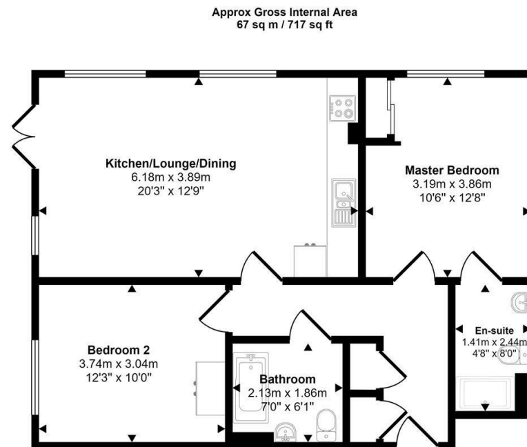
Floorplan
