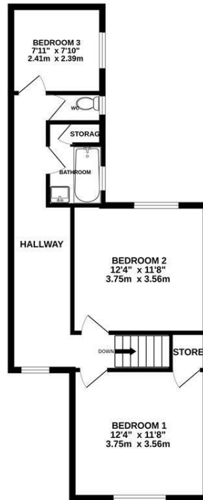
1ST FLOOR
