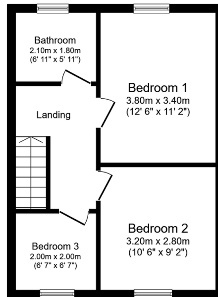
First Floor Floor area 37.4 sq.m. (403 sq.ft.)
