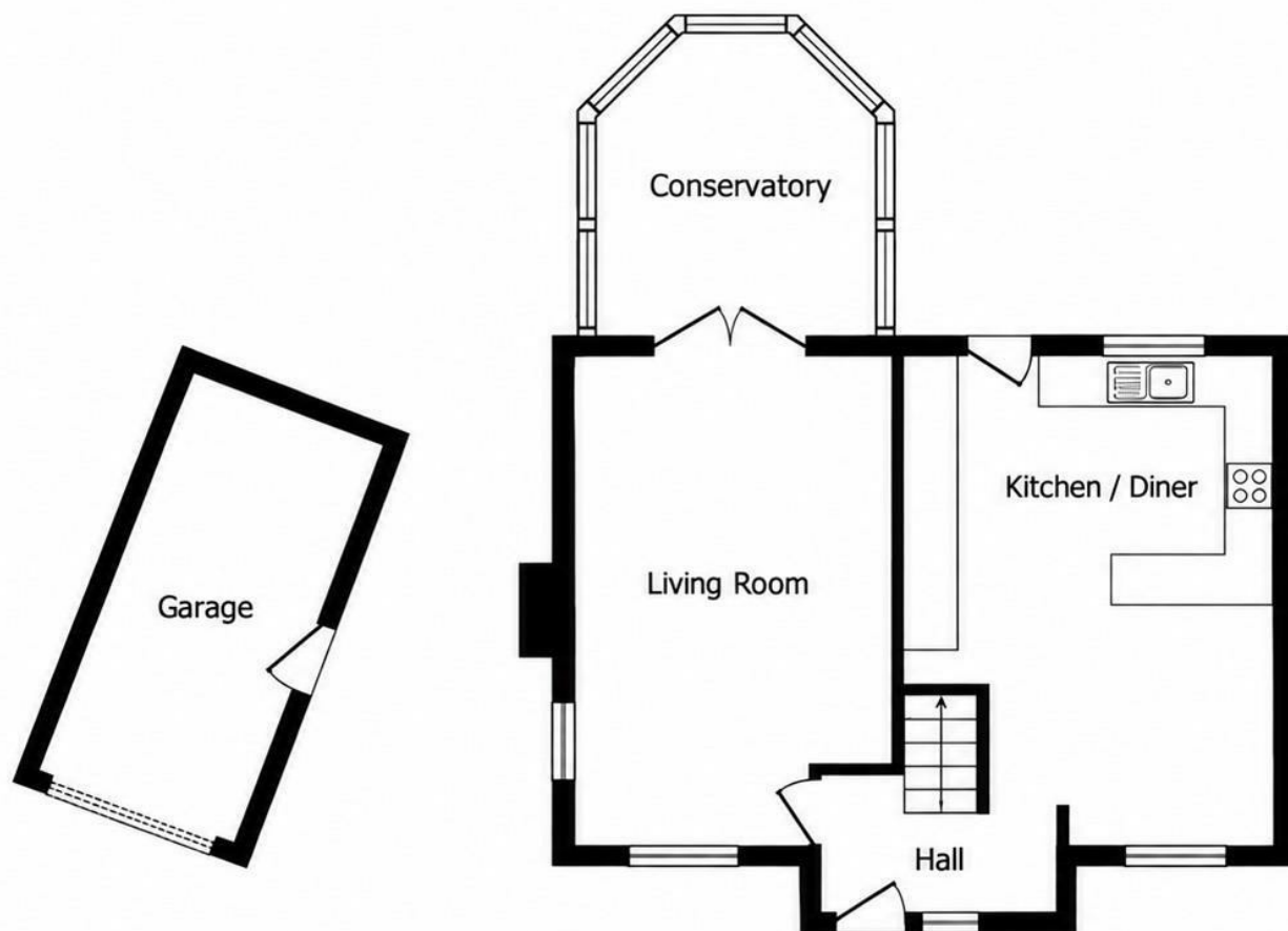
Ground Floor
