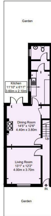
Ground Floor
