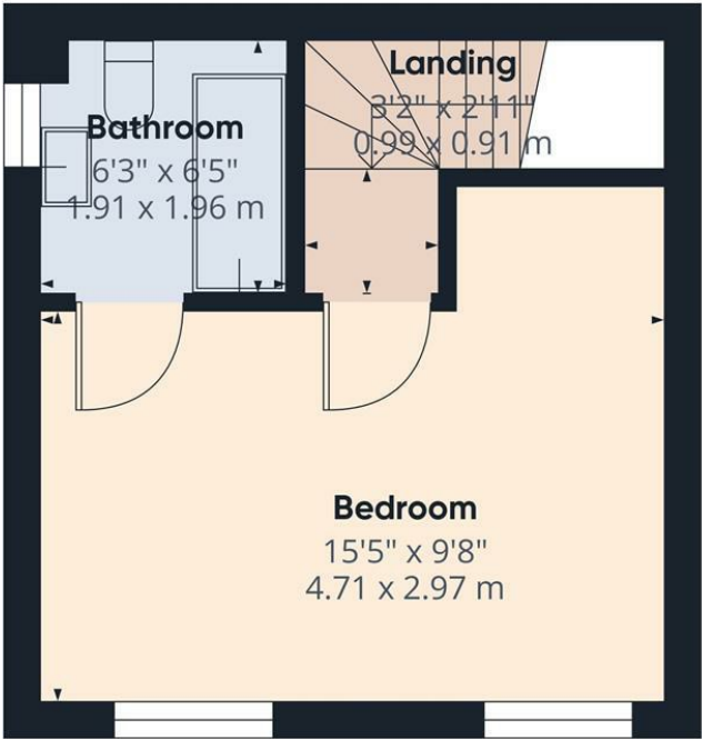
Floor 1
