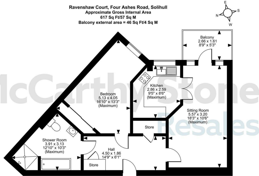
First Floor FOR ILLUSTRATIVE PURPOSES ONLY - NOT TO SCALE The position & size of doors, windows, appliances and other features are approximate only. © ehouse. Unauthorised reproduction prohibited. Drawing ref. dig/8632932/LPV
