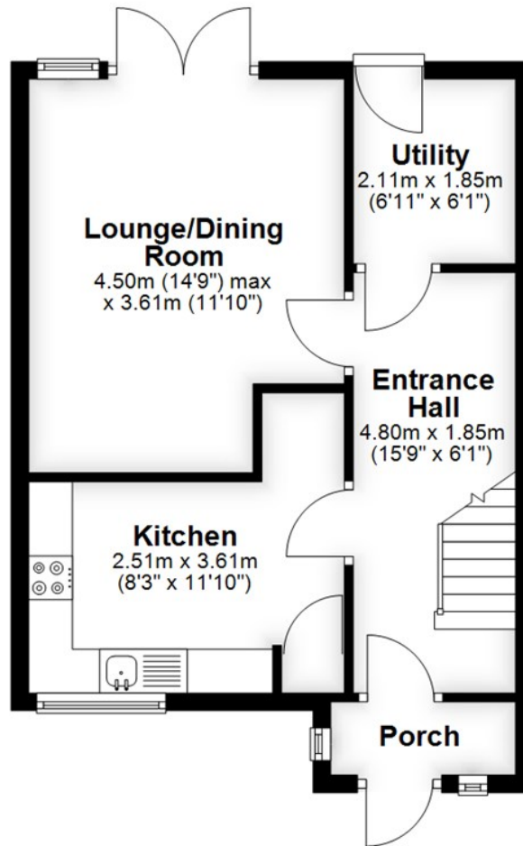
Ground Floor Approx. 41.3 sq. metres (444.6 sq. feet)
