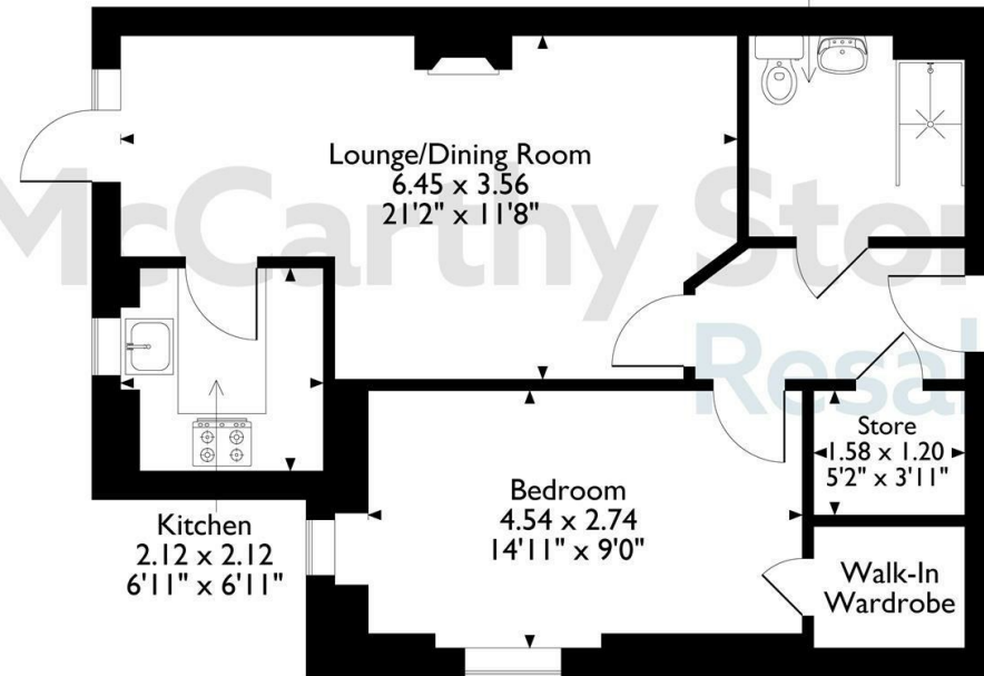
The position & size of doors, windows, appliances and other features are approximate only. © ehouse. Unauthorised reproduction prohibited. Drawing ref. dig/8682568/DST.
