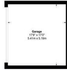
Garage Approximate Floor Area 302 sq.ft (28.07 sq.m)
