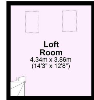
First Floor Approx. 16.7 sq. metres (180.3 sq. feet)
