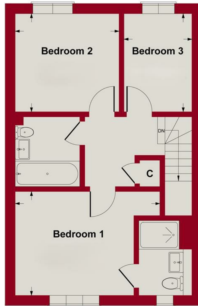
FIRST FLOOR
