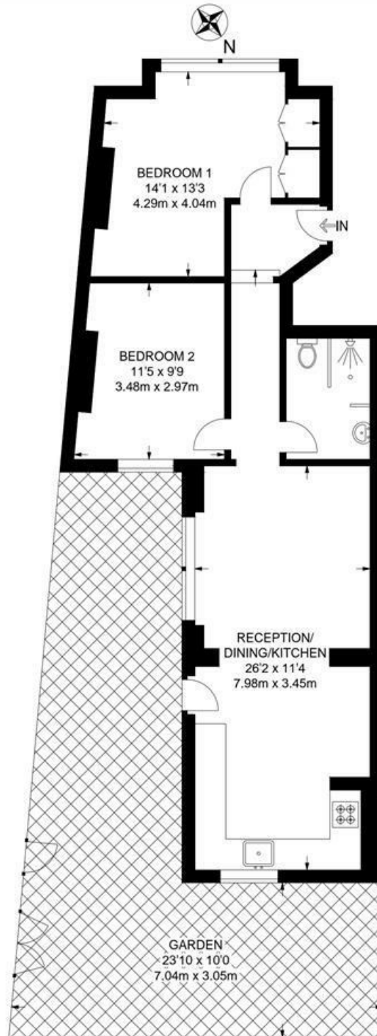
GROUND FLOOR
