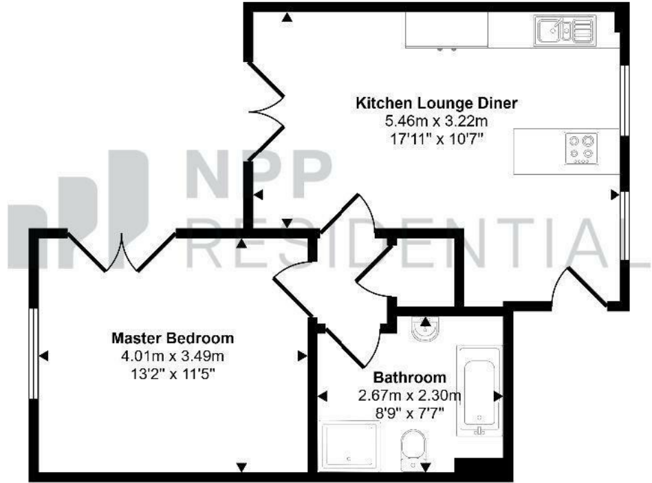
Floorplan
