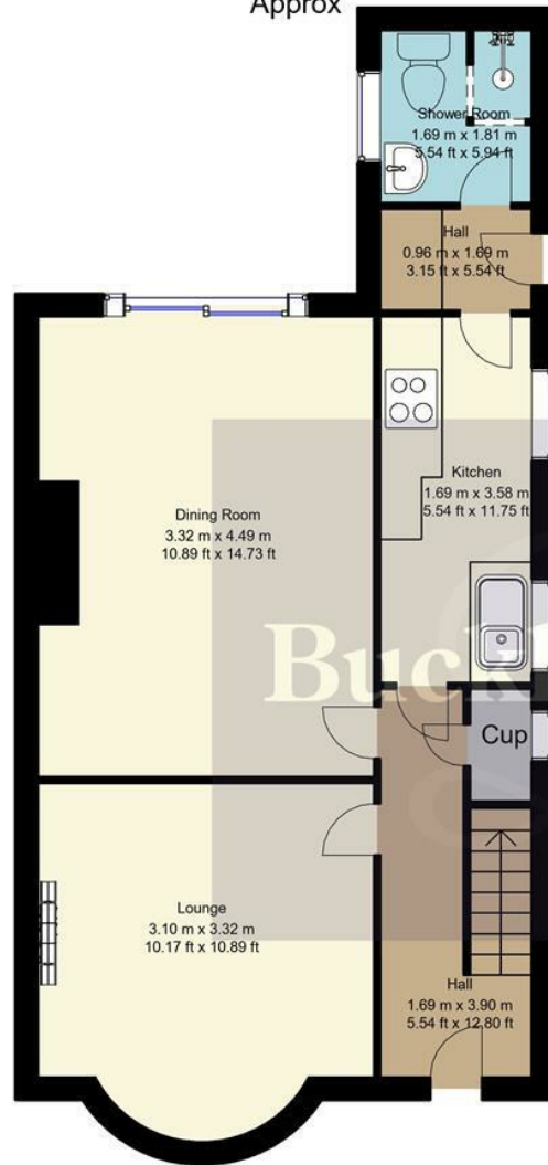
Ground Floor 47 sq.mt / 505.9 sq.ft Approx
