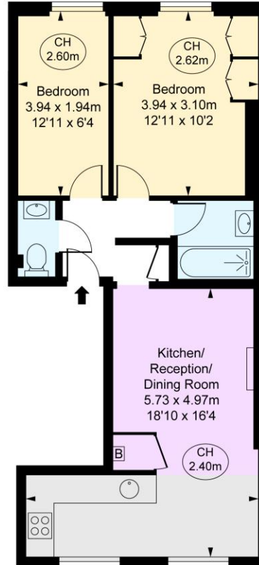
Second Floor
