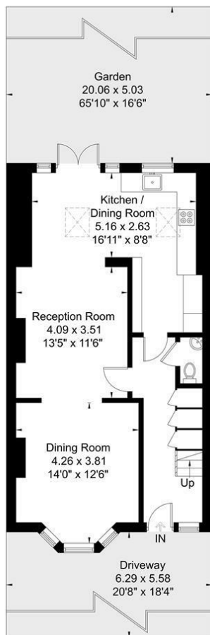
Ground Floor 64.1 sq m / 690 sq ft
