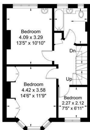
First Floor 48.8 sq m / 525 sq ft
