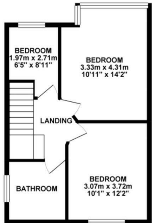
1ST FLOOR 40.66 sq. m. ( 437.65 sq. ft. )
