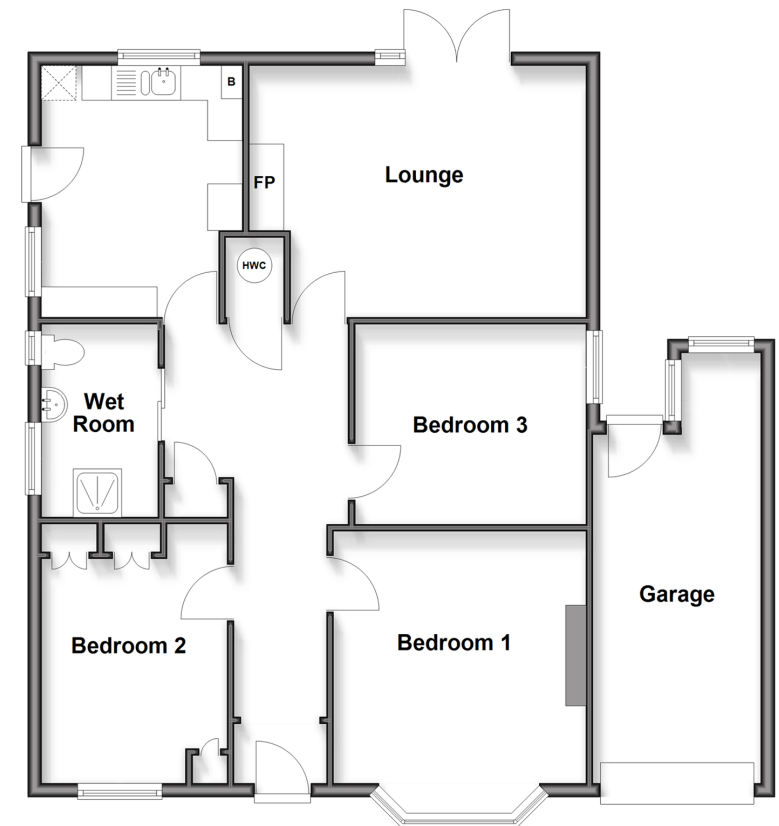
Ground Floor Approx. 96.0 sq. metres (1033.6 sq. feet)
