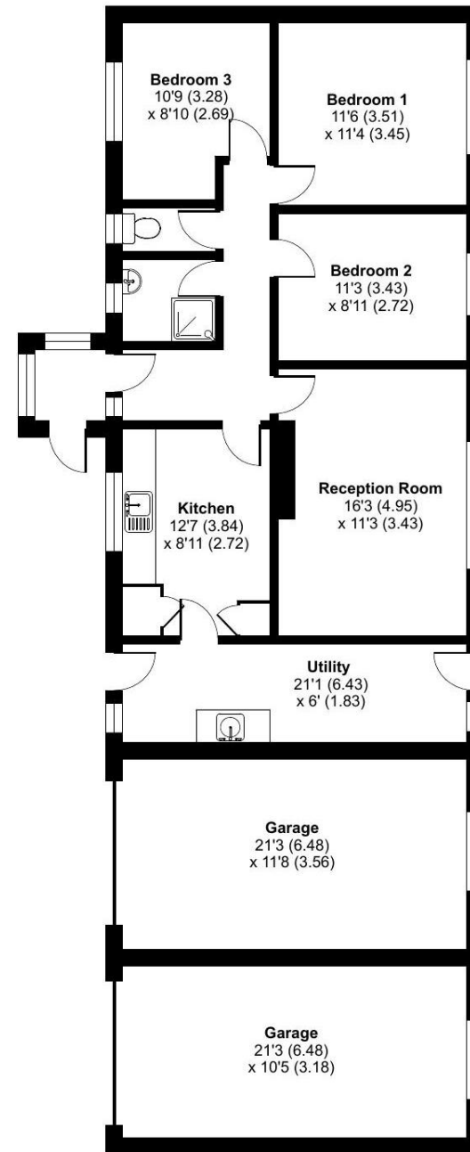
GROUND FLOOR
