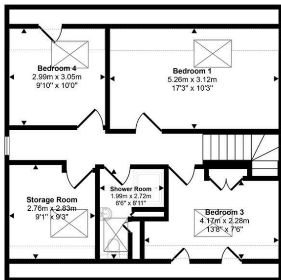
First Floor Approx 69 sq m / 744 sq ft
