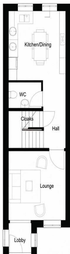
House Type B – Ground Floor Plan 1:50
