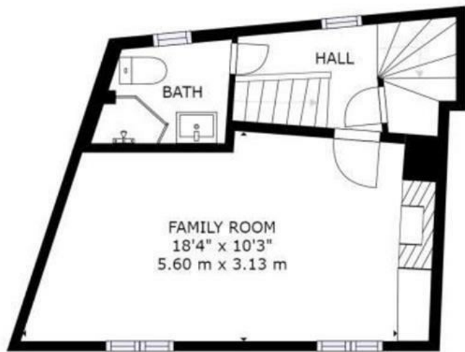
FLOOR 2
