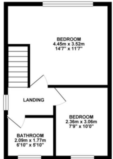
1ST FLOOR 29.24 sq. m. ( 314.73 sq. ft. )
