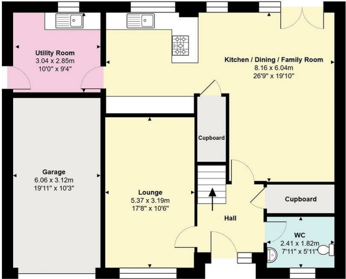
Ground Floor Approximate Area: 82.4 m² ... 887 ft²
