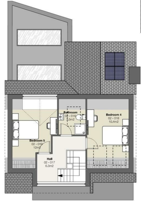
3 Second Floor Plan Scale: 1:100
