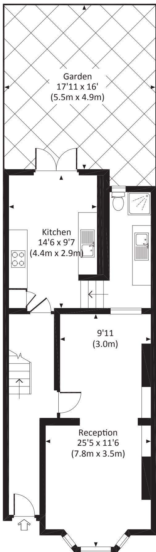
GROUND FLOOR
