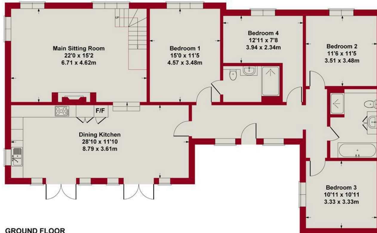
GROUND FLOOR
