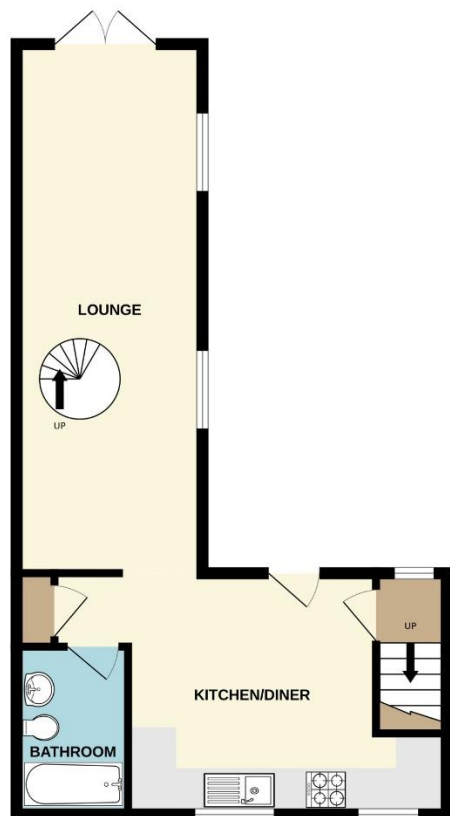
GROUND FLOOR 484 sq.ft. (44.9 sq.m.) approx.
