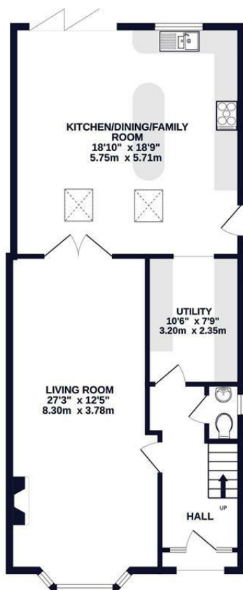
GROUND FLOOR 850 sq.ft. (78.9 sq.m.) approx.
