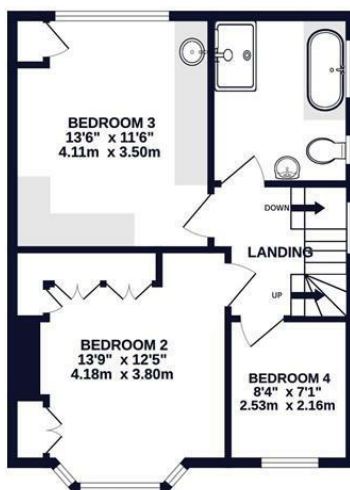
1ST FLOOR 507 sq.ft. (47.1 sq.m.) approx.
