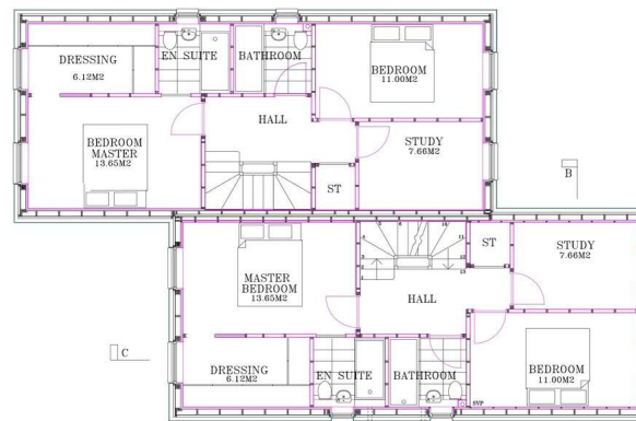
FIRST FLOOR PLAN 60.00M2
