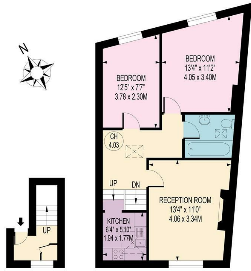
SECOND FLOOR
