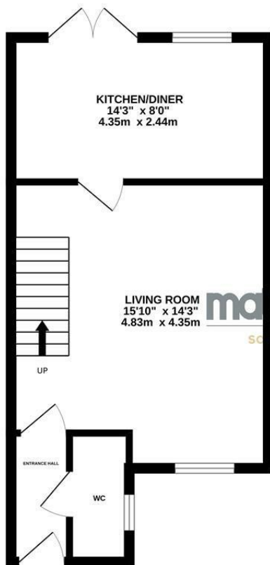
GROUND FLOOR 374 sq.ft. (34.8 sq.m.) approx.
