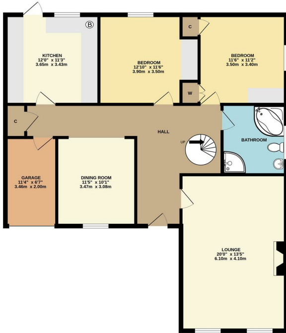
GROUND FLOOR 1147 sq.ft. (106.6 sq.m.) approx.
