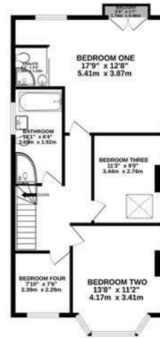
1ST FLOOR 714 sq.ft. (66.3 sq.m.) approx.
