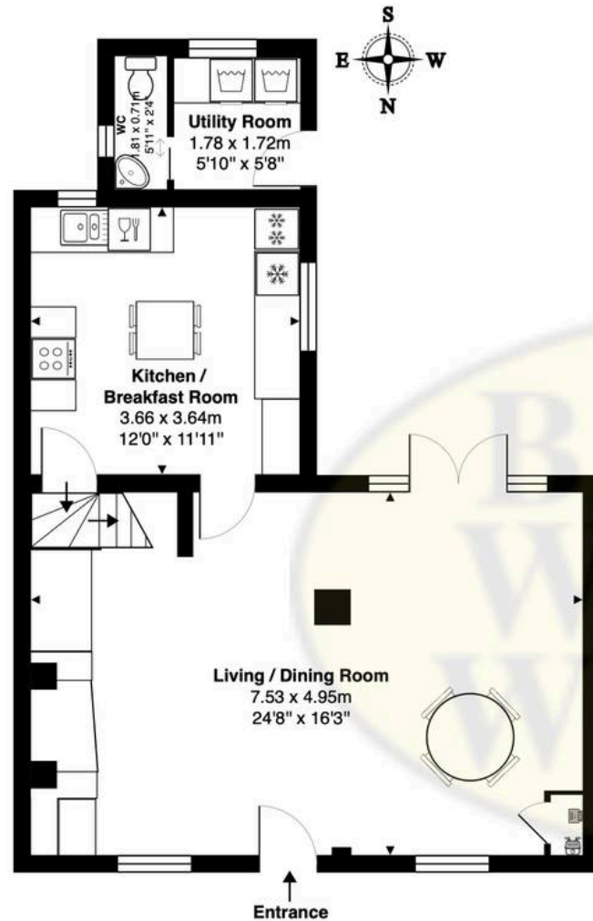
Ground Floor Floor Area: 56.7 m 2 ... 610 ft 2
