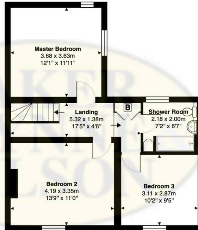
First Floor Floor Area: 52.1 m 2 ... 560 ft 2
