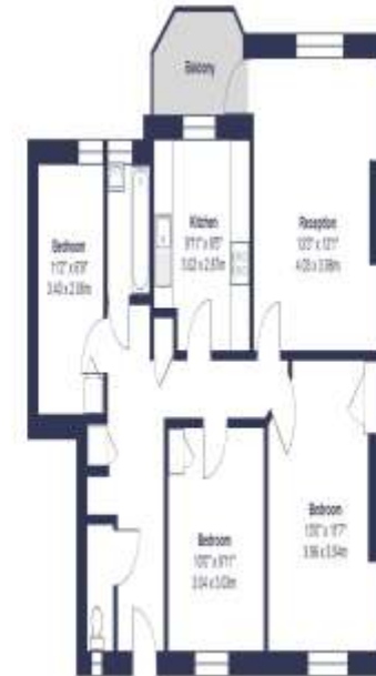
1st Floor
