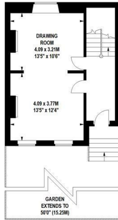
Ground Floor
