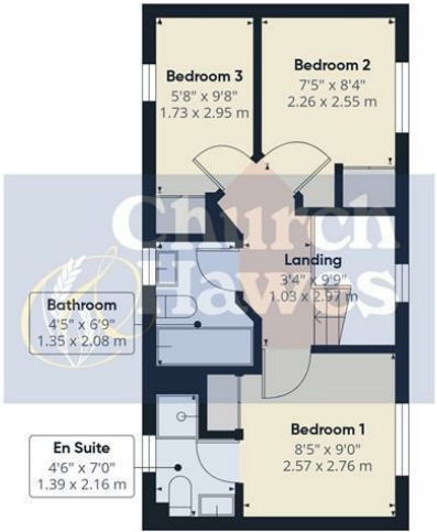
Floor 1 Building 1
