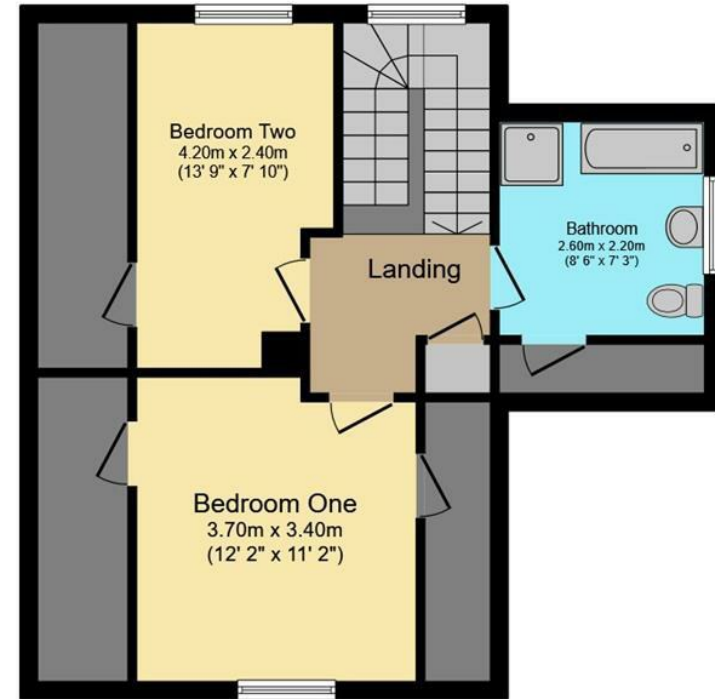
First Floor Floor area 39.6 sq.m. (426 sq.ft.)
