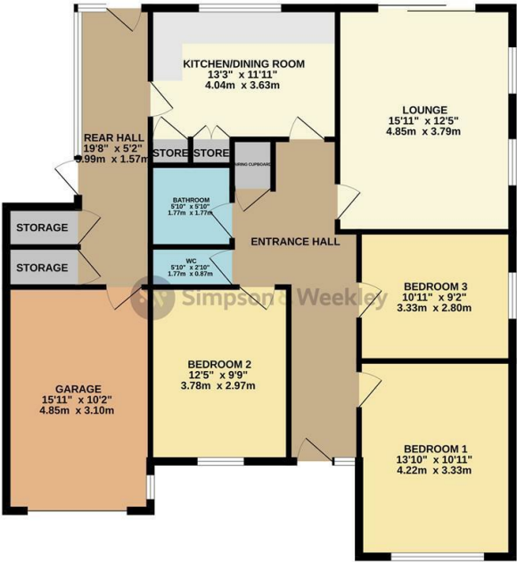
GROUND FLOOR 1198 sq.ft. (111.3 sq.m.) approx.
