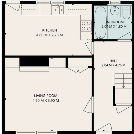
1ST FLOOR
