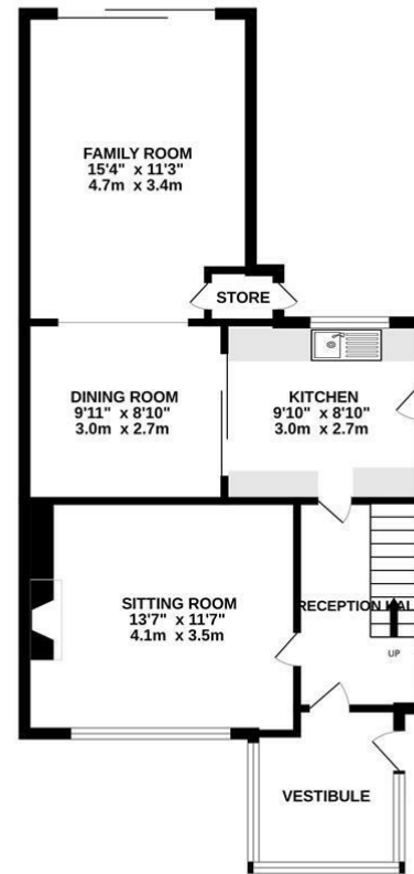
GROUND FLOOR 616 sq.ft. (57.3 sq.m.) approx.
